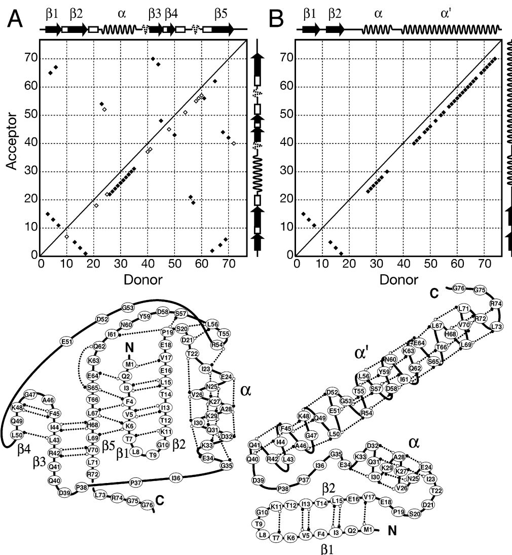
FIGURE 1: Hydrogen bond topologies as derived by detected ^3J_{NC'} H-bond correlations for ubiquitin in the native state (A) and in the A-state (B). Top: two-dimensional maps representing the detected ^3J_{NC'} scalar correlations (filled diamonds). Secondary structure elements are indicated as filled arrows for \beta -strands, solid wavy lines for \alpha -helices, dashed wavy lines for 3_{10} -helices, and open boxes for \beta -turns. For the native state (A) open diamonds represent H-bonds, which were not detected by ^3J_{NC'} correlations but which are present in the ubiquitin crystal structure (1UBQ) (47) with d_{OH} < 2.5 Å and NH\cdots O angles > 120^\circ . Bottom: H-bond topology diagrams derived for the two states based on detected ^3J_{NC'} correlations. The H-bonds are depicted by a dotted line between the amide proton donors (filled hexagons) and the oxygen acceptors (open hexagons).
